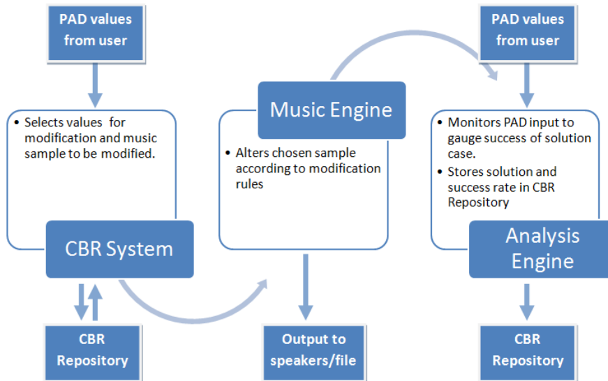
Figure 2. Affective Music Synthesis Design Overview
