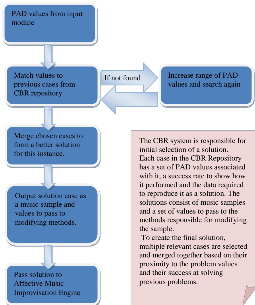
Figure 3. CBR System Flow Diagram
