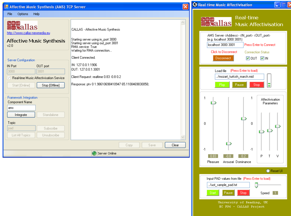
Figure 4. AMS Server and RMA GUIs
