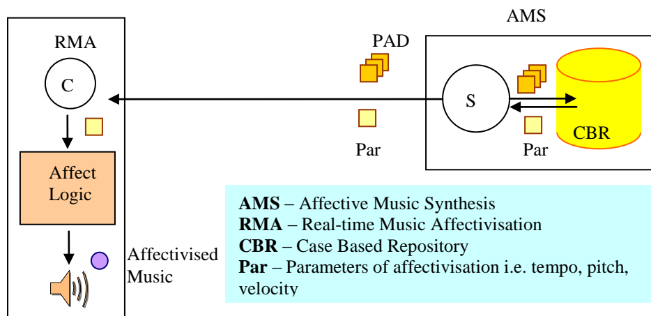
Figure 5. TCP communication between RMA and AMS
