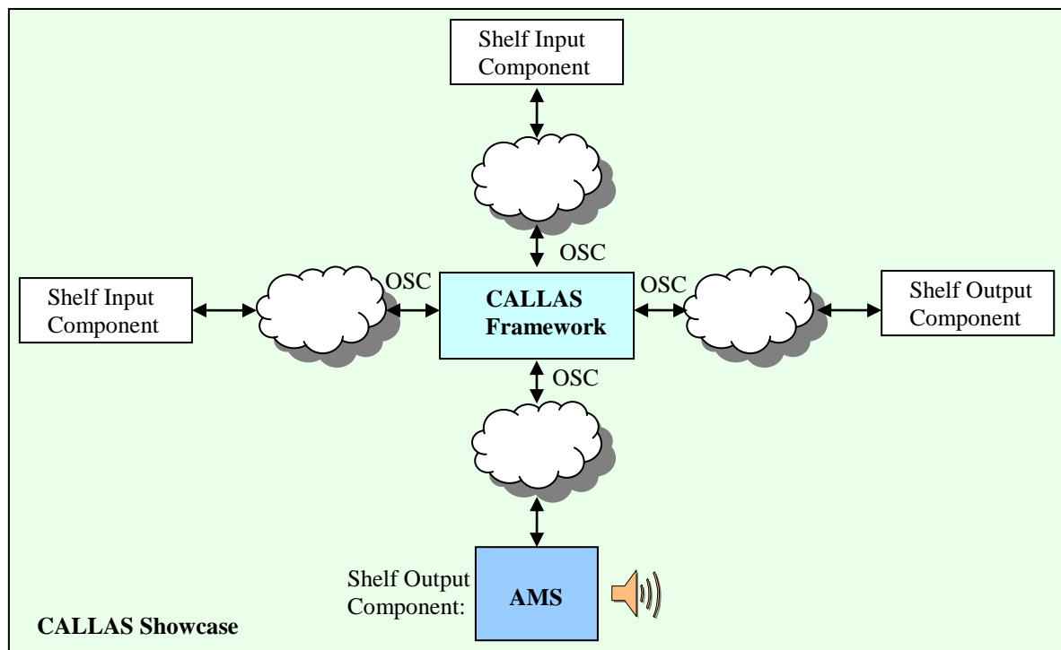
Figure 6. OSC Integration of AMS with CALLAS Framework
